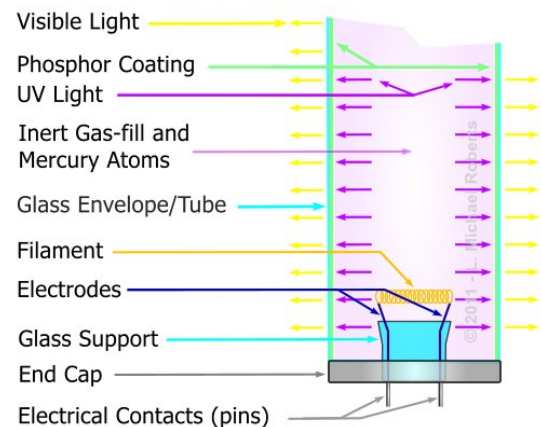
FLUORESCENT LAMP DIAGRAM
